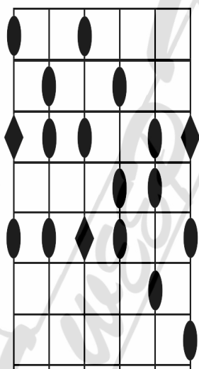
5. Mixolidia b6
